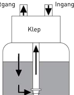
C2 PEKELAANZUIGING & TRAGE SPOELING
